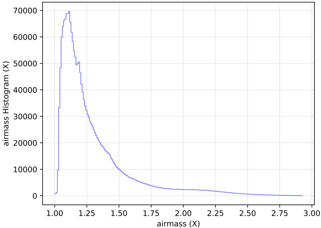
internal_u_expt60_nscale0.9v3.4_10yrs WFD all bands: airmass Histogram
