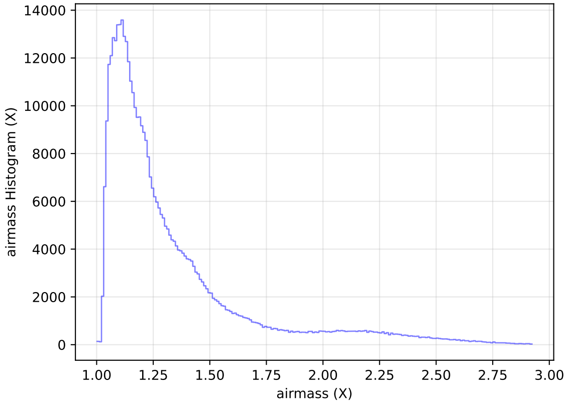
internal_u_expt60_nscale0.9v3.4_10yrs All sky z band: airmass Histogram
