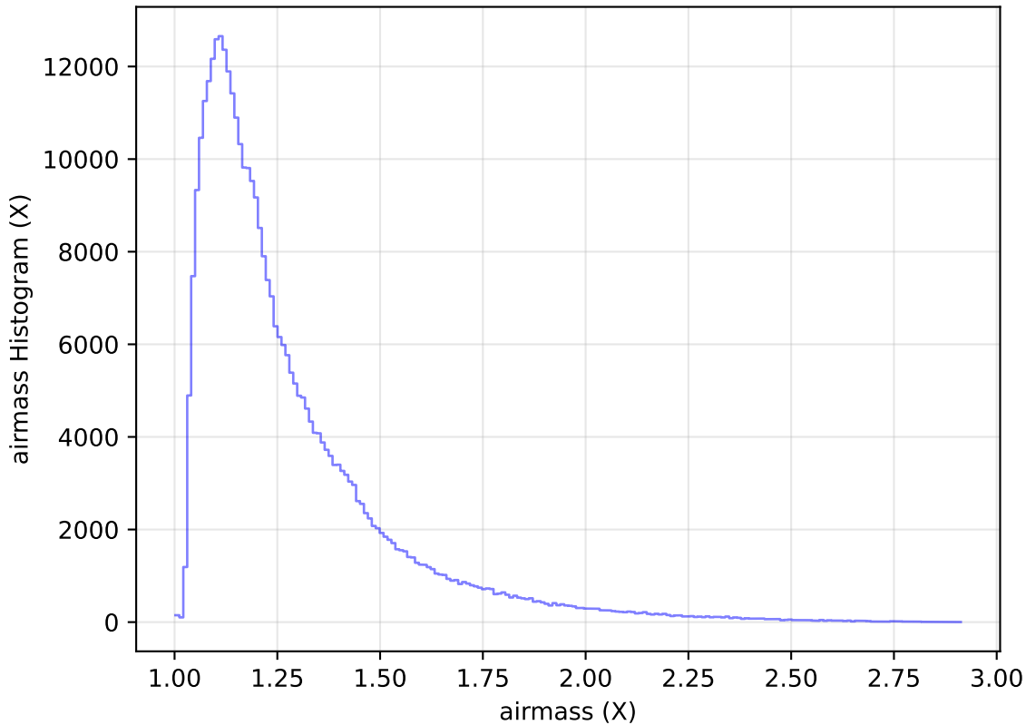
internal_u_expt60_nscale0.9v3.4_10yrs All sky y band: airmass Histogram
