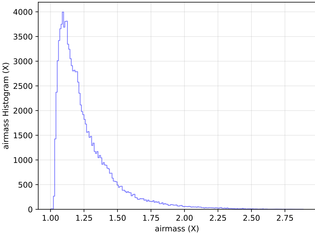
internal_u_expt60_nscale0.9v3.4_10yrs All sky u band: airmass Histogram
