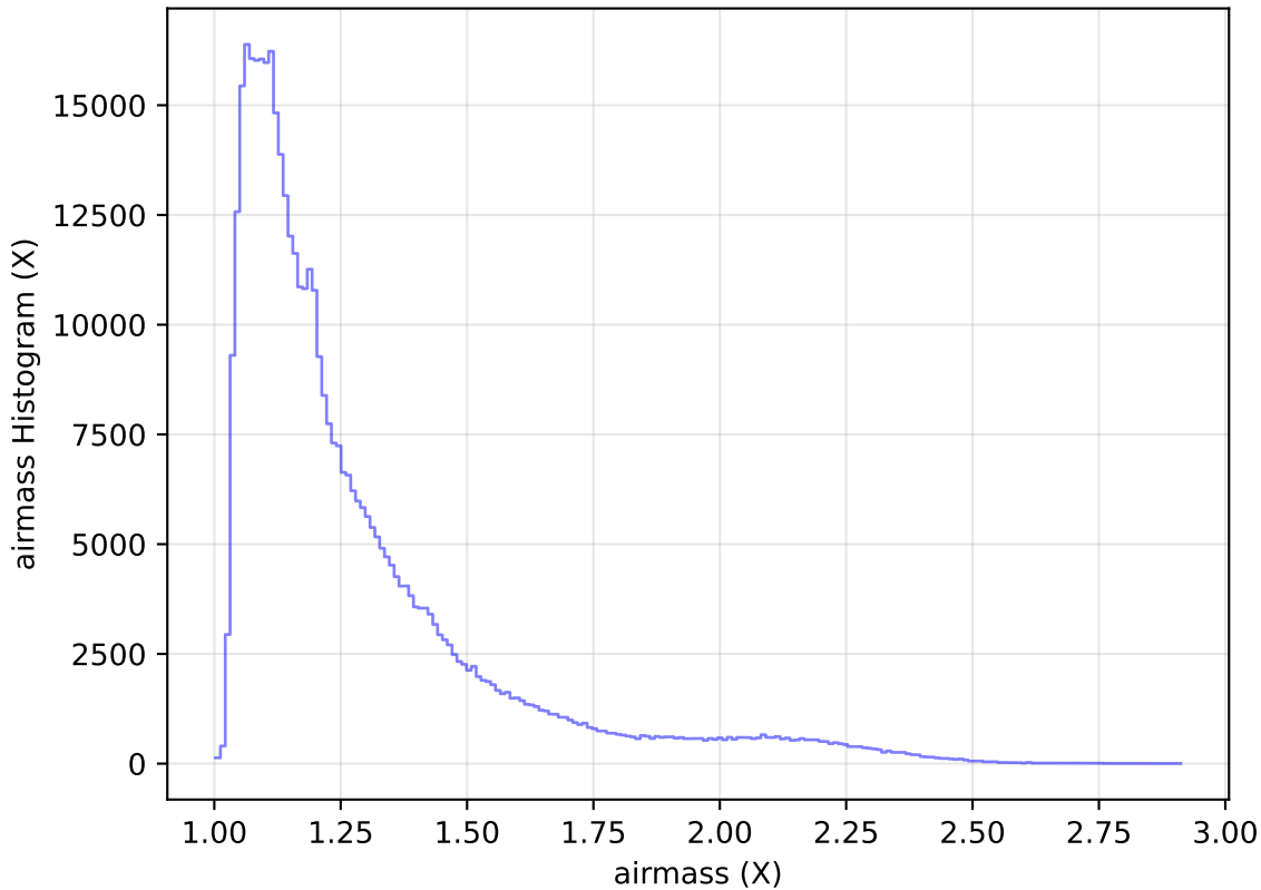
internal_u_expt60_nscale0.9v3.4_10yrs All sky r band: airmass Histogram
