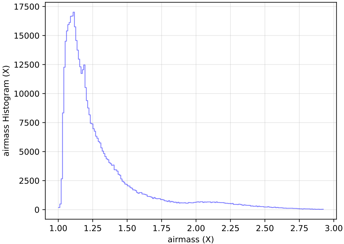
internal_u_expt60_nscale0.9v3.4_10yrs All sky i band: airmass Histogram
