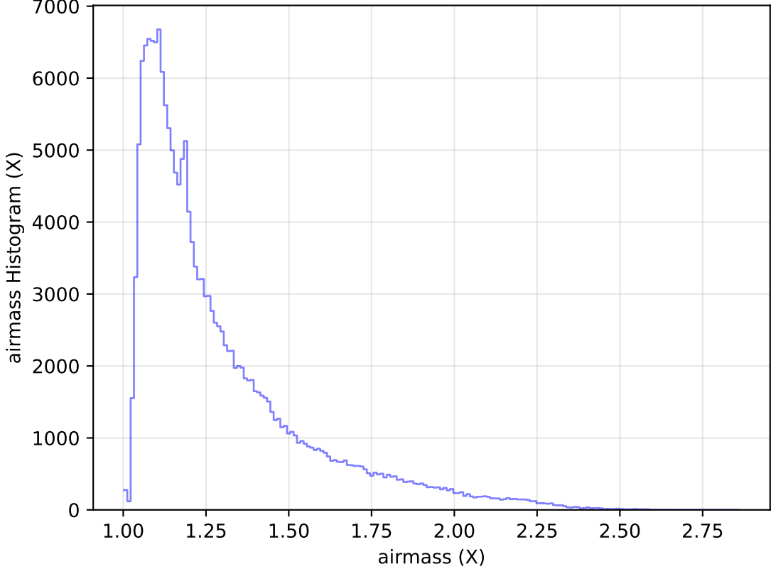
internal_u_expt60_nscale0.9v3.4_10yrs All sky g band: airmass Histogram
