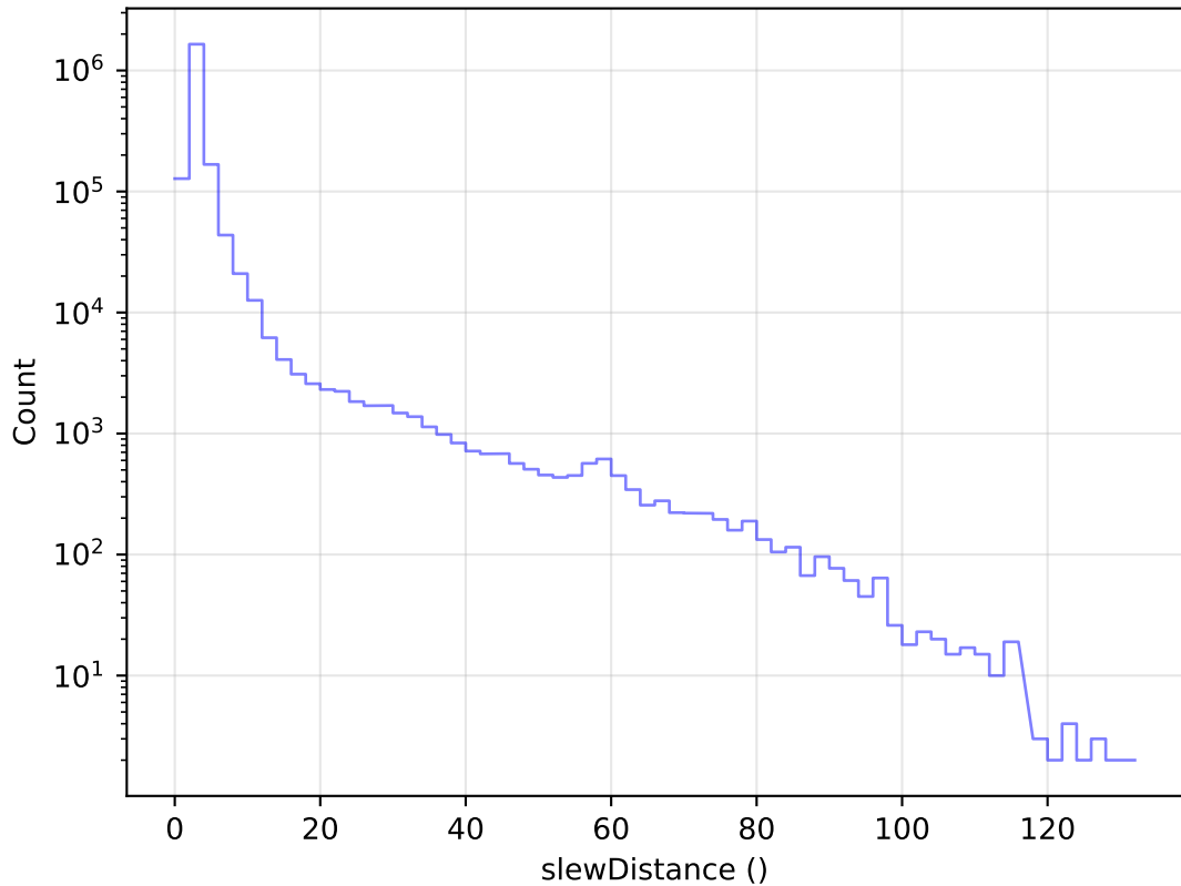
internal_u_expt60_nscale0.9v3.4_10yrs All visits: Slew Distance Histogram
