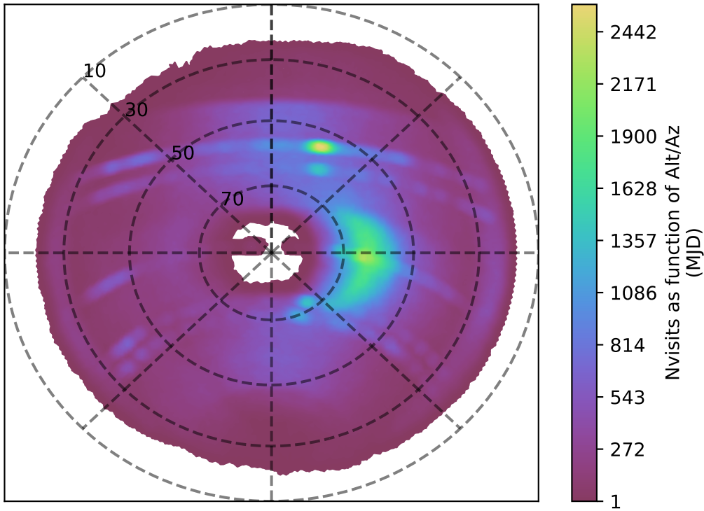
internal_u_expt60_nscale0.9v3.4_10yrs z band: Nvisits as function of Alt/Az
