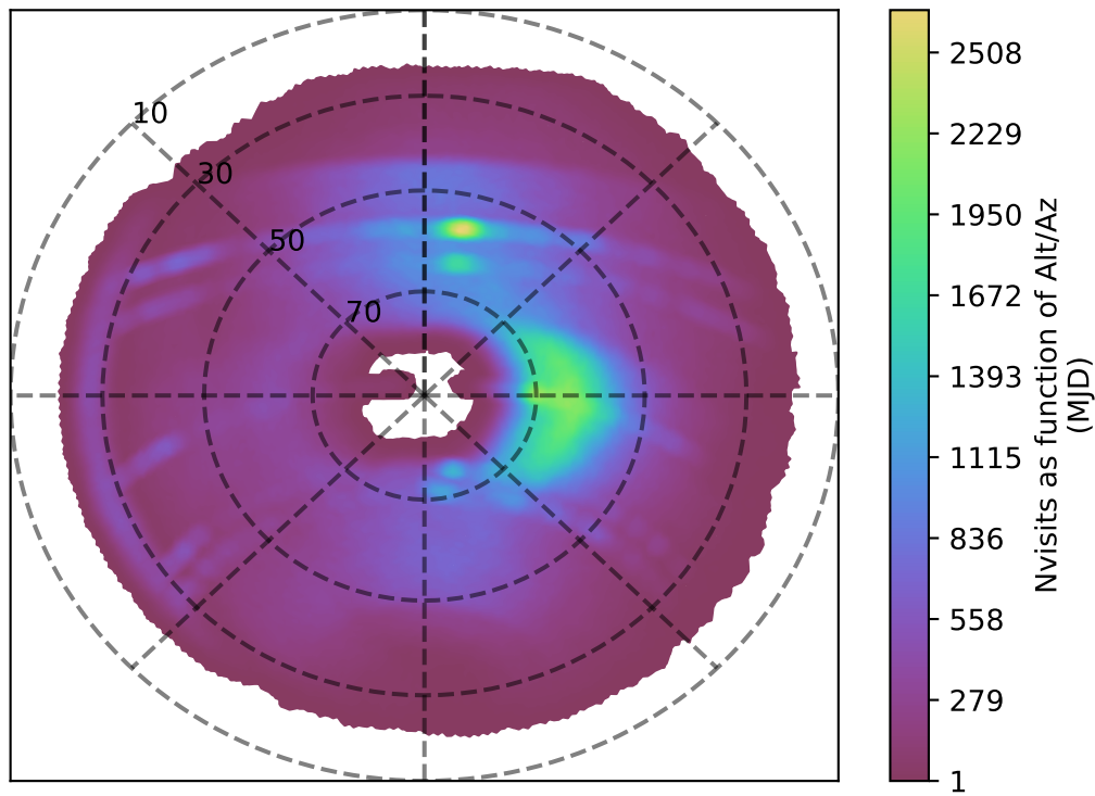
internal_u_expt60_nscale0.9v3.4_10yrs r band: Nvisits as function of Alt/Az
