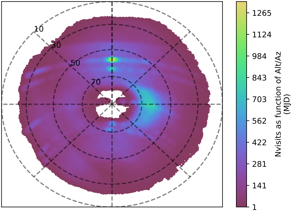
internal_u_expt60_nscale0.9v3.4_10yrs g band: Nvisits as function of Alt/Az
