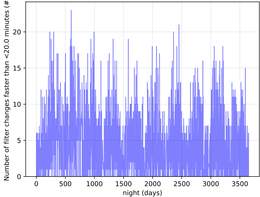
internal_u_expt60_nscale0.9v3.4_10yrs Per Night: Number of filter changes faster than <20.0 minutes
