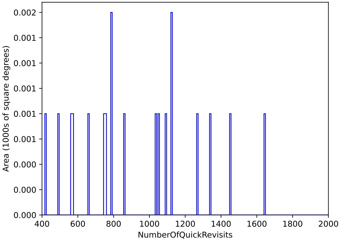
internal_u_expt60_nscale0.9v3.4_10yrs WFD: NumberOfQuickRevisits
