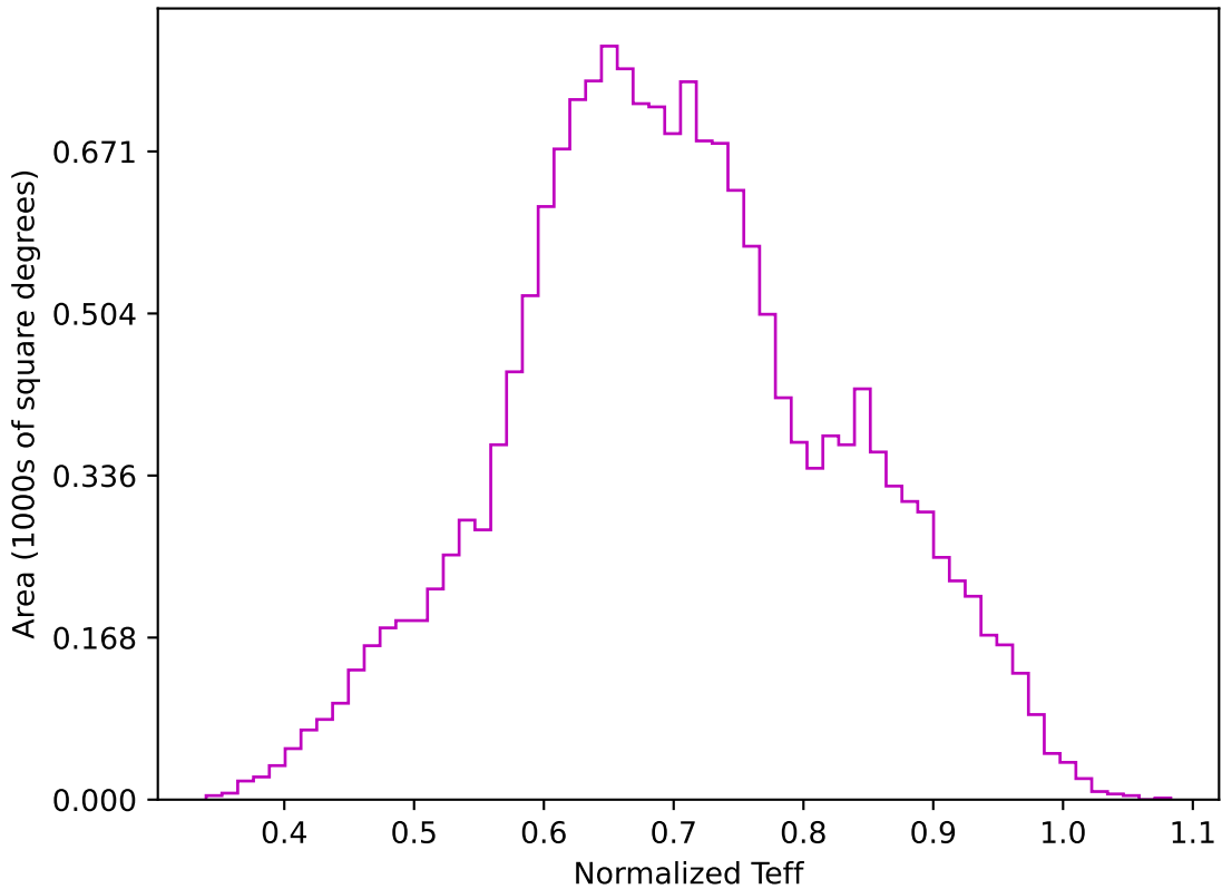
internal_u_expt60_nscale0.9v3.4_10yrs WFD z band: Normalized Teff
