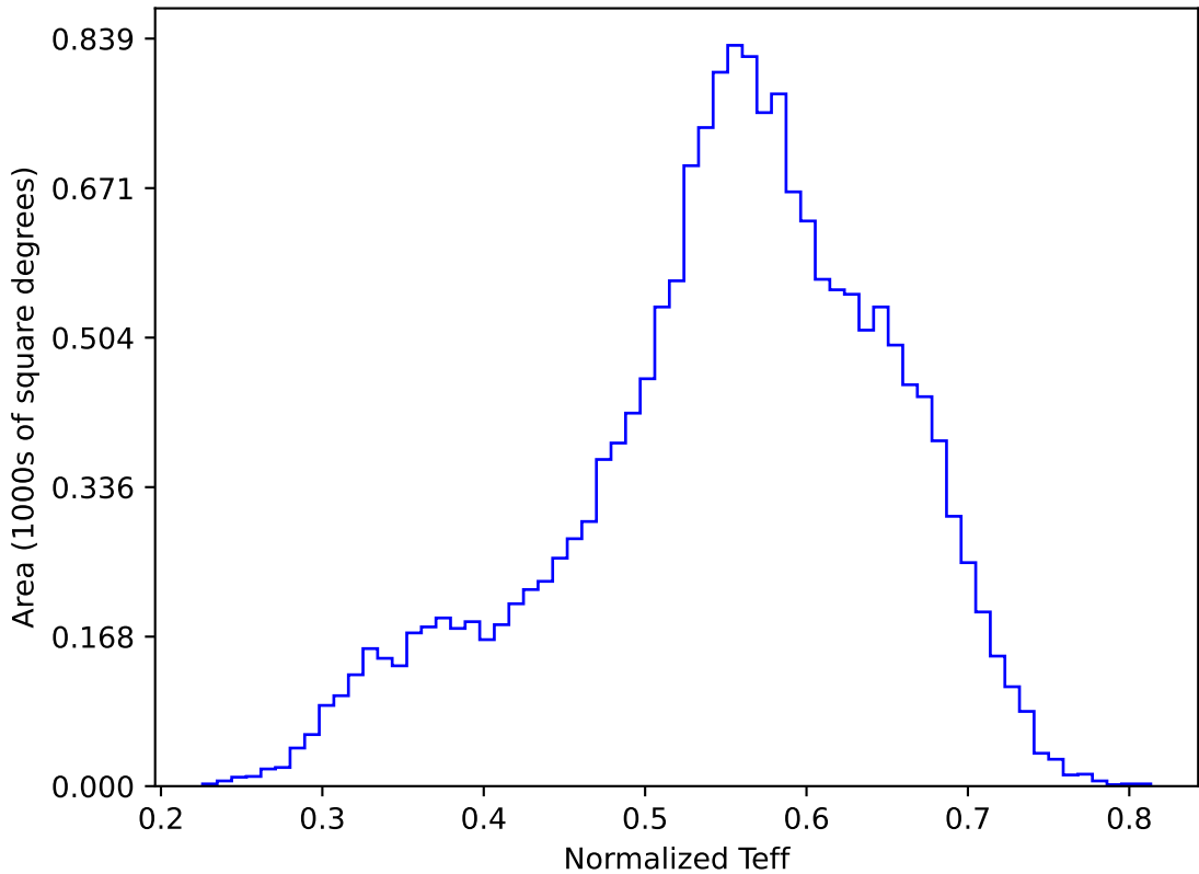
internal_u_expt60_nscale0.9v3.4_10yrs WFD y band: Normalized Teff
