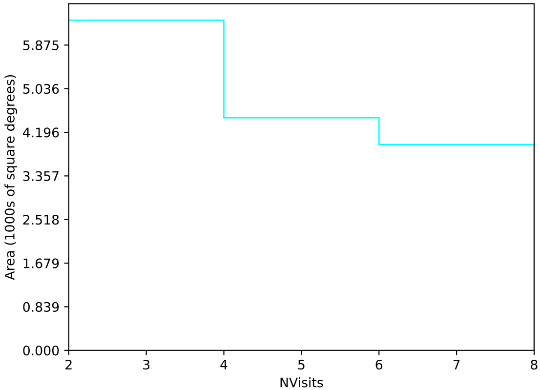
internal_u_expt60_nscale0.9v3.4_10yrs Yr 3-4 u band: NVisits
