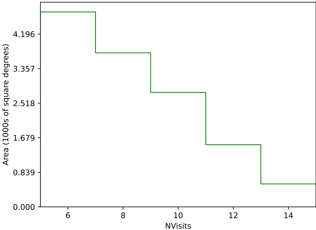
internal_u_expt60_nscale0.9v3.4_10yrs Yr 3-4 g band: NVisits
