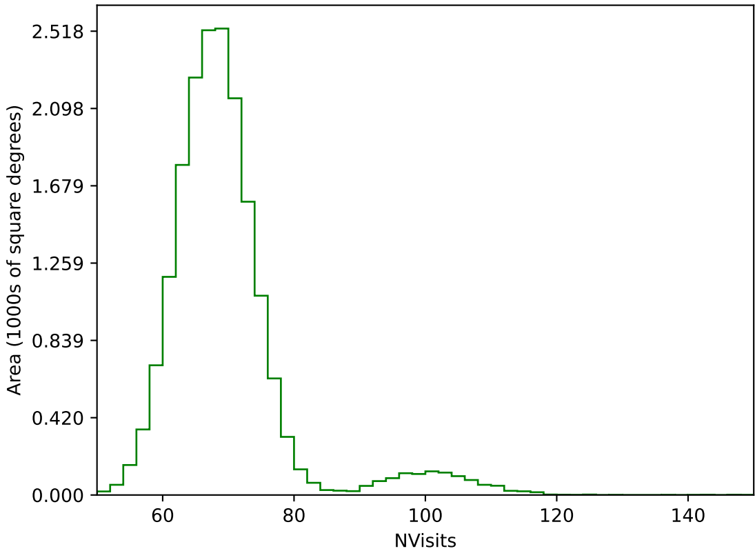
internal_u_expt60_nscale0.9v3.4_10yrs WFD g band: NVisits
