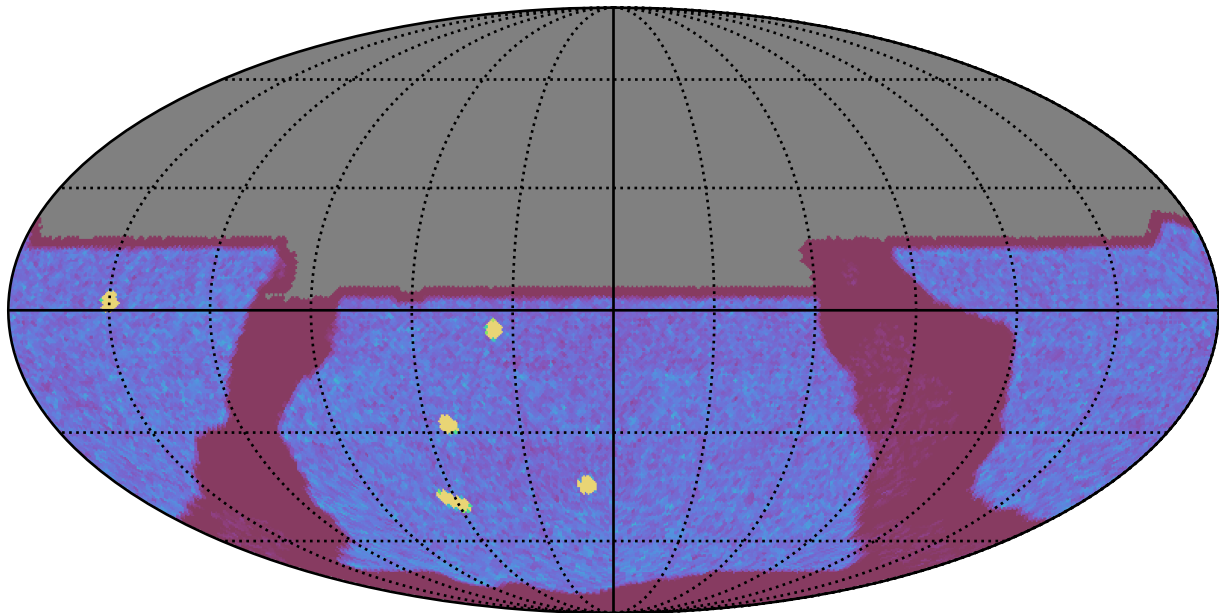
internal_u_expt60_nscale0.9v3.4_10yrs All sky y band: NVisits
