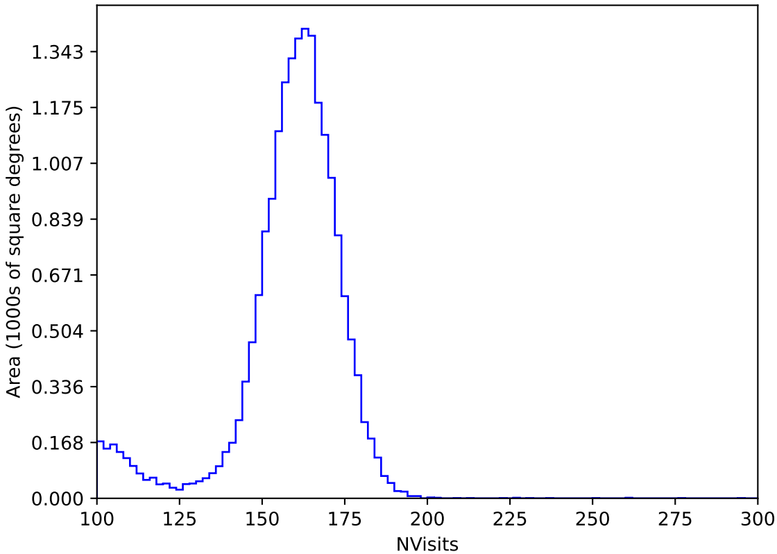
internal_u_expt60_nscale0.9v3.4_10yrs All sky y band: NVisits
