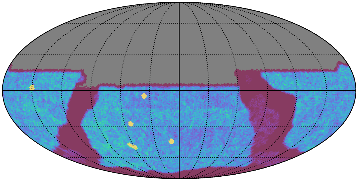
internal_u_expt60_nscale0.9v3.4_10yrs All sky u band: NVisits
