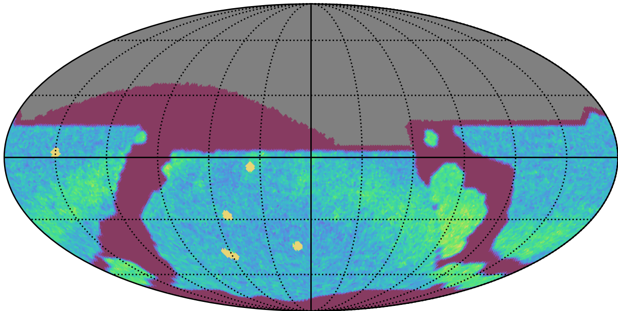
internal_u_expt60_nscale0.9v3.4_10yrs All sky r band: NVisits
