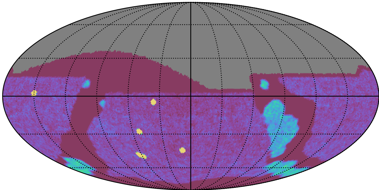
internal_u_expt60_nscale0.9v3.4_10yrs All sky g band: NVisits
