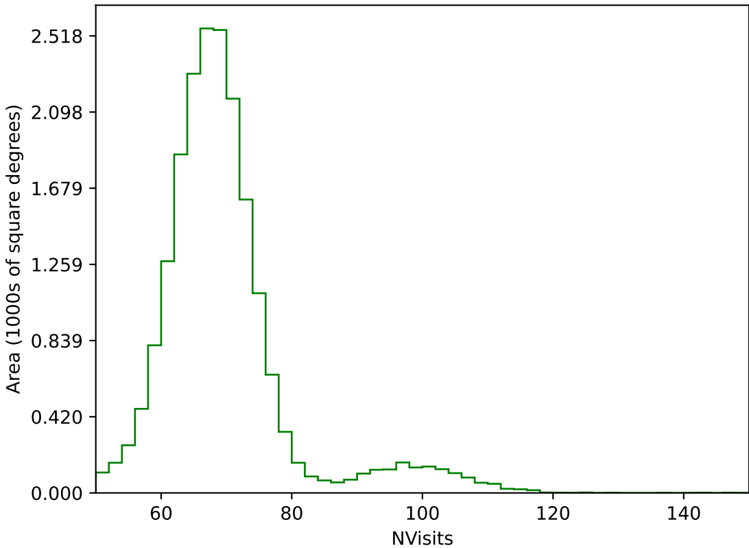
internal_u_expt60_nscale0.9v3.4_10yrs All sky g band: NVisits
