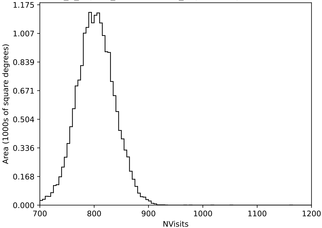
internal_u_expt60_nscale0.9v3.4_10yrs All sky all bands: NVisits
