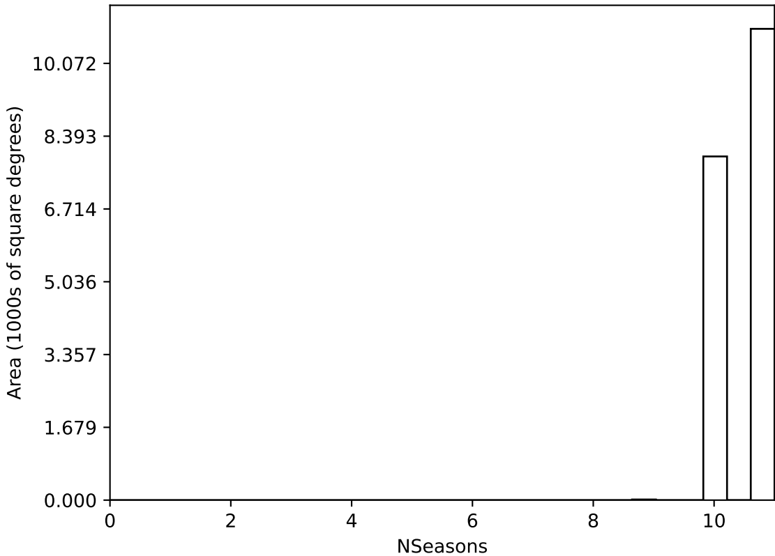
internal_u_expt60_nscale0.9v3.4_10yrs WFD all bands: NSeasons
