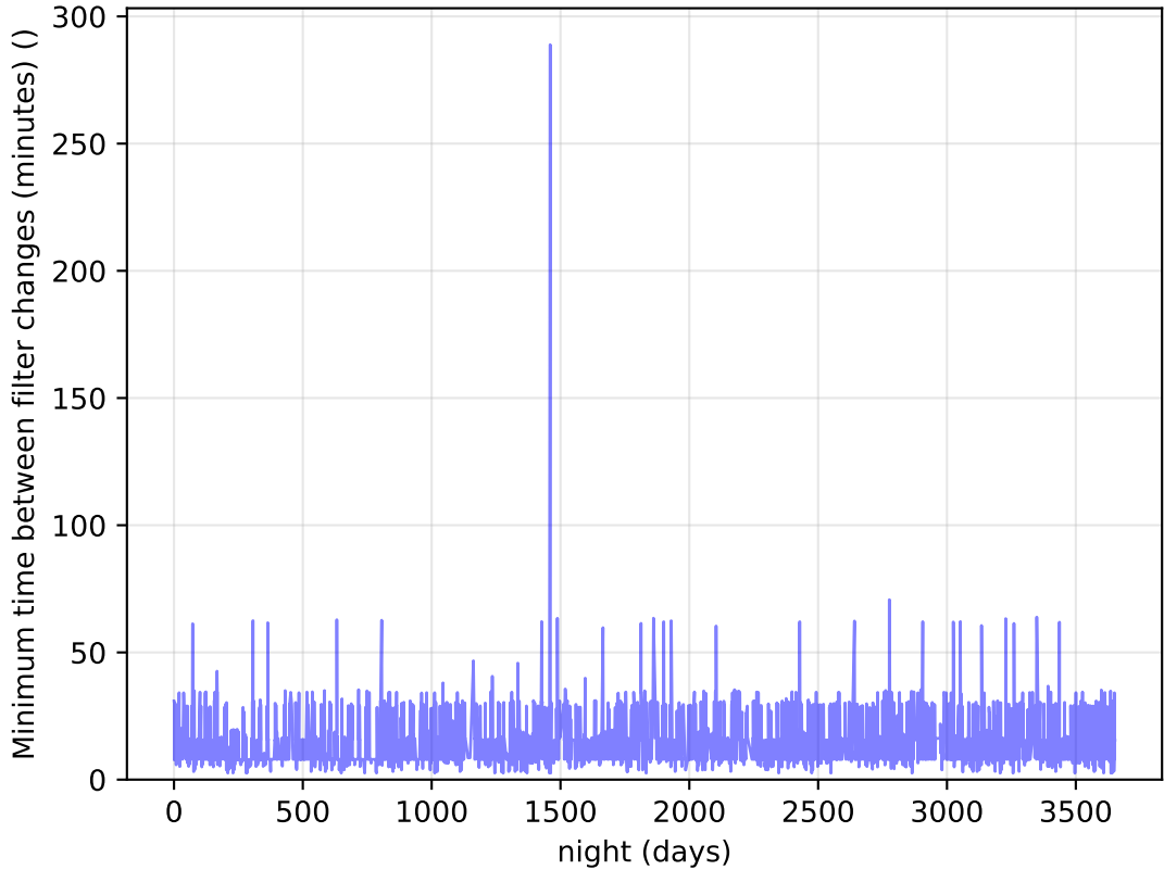
internal_u_expt60_nscale0.9v3.4_10yrs Per Night: Minimum time between filter changes (minutes)
