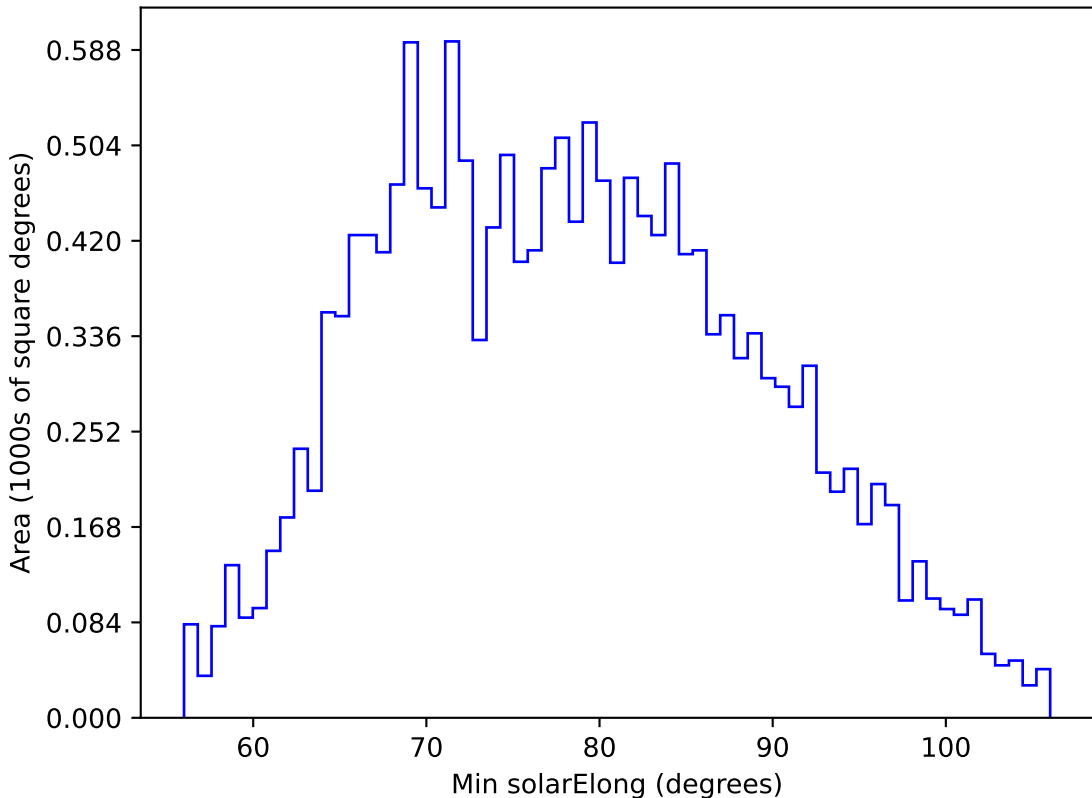
internal_u_expt60_nscale0.9v3.4_10yrs WFD u band: Min solarElong
