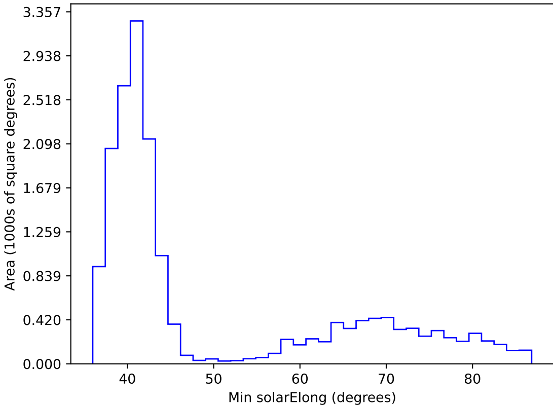
internal_u_expt60_nscale0.9v3.4_10yrs WFD i band: Min solarElong
