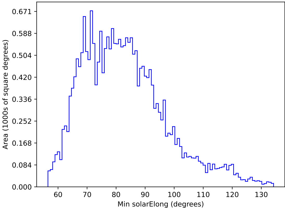
internal_u_expt60_nscale0.9v3.4_10yrs All sky u band: Min solarElong
