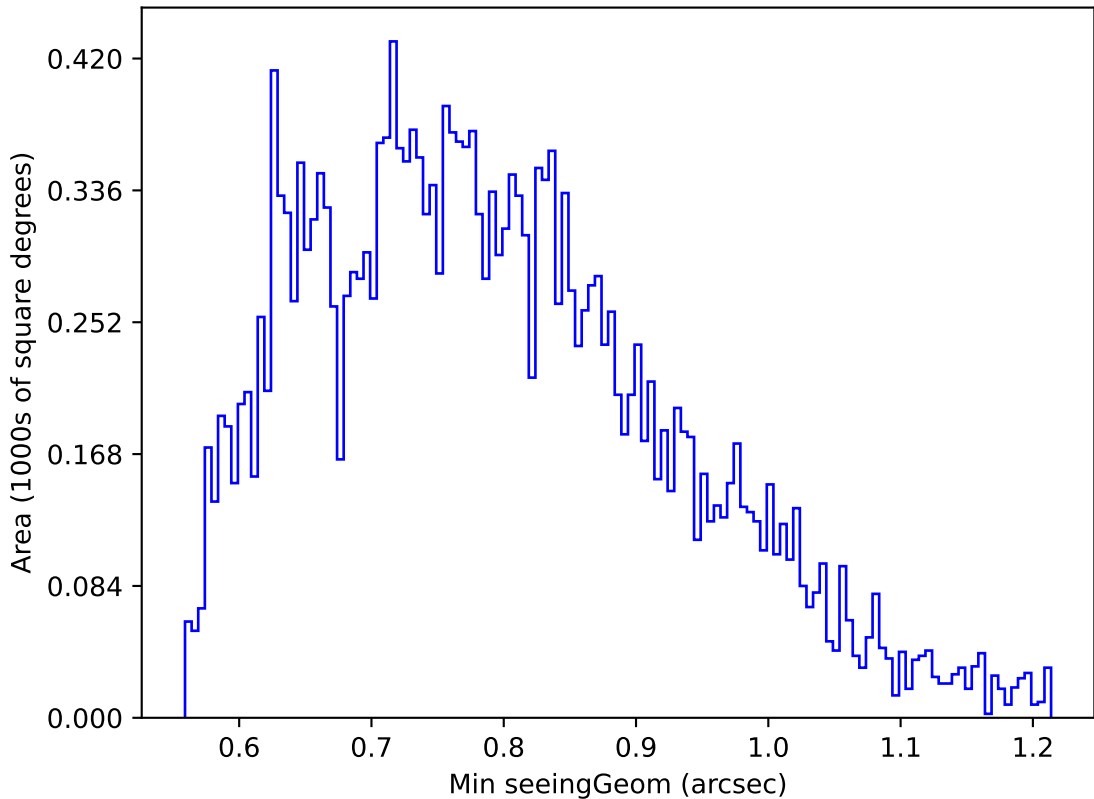
internal_u_expt60_nscale0.9v3.4_10yrs Yr 1 u band: Min seeingGeom
