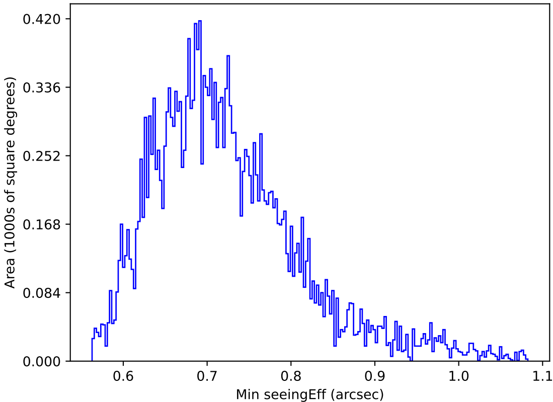
internal_u_expt60_nscale0.9v3.4_10yrs Yr 1 y band: Min seeingEff
