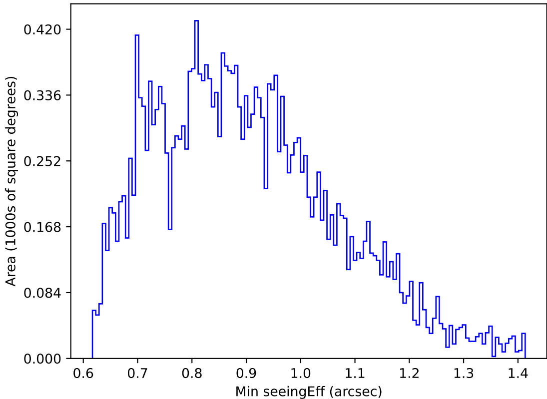
internal_u_expt60_nscale0.9v3.4_10yrs Yr 1 u band: Min seeingEff
