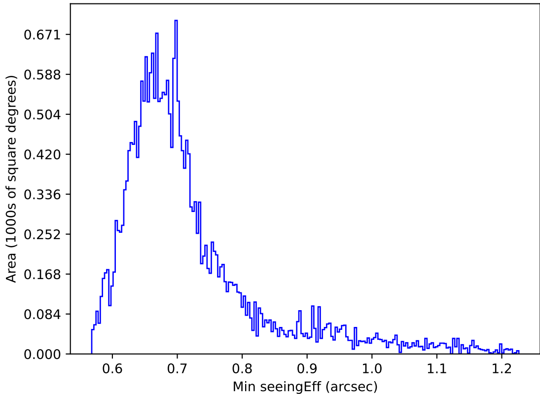
internal_u_expt60_nscale0.9v3.4_10yrs Yr 1 i band: Min seeingEff
