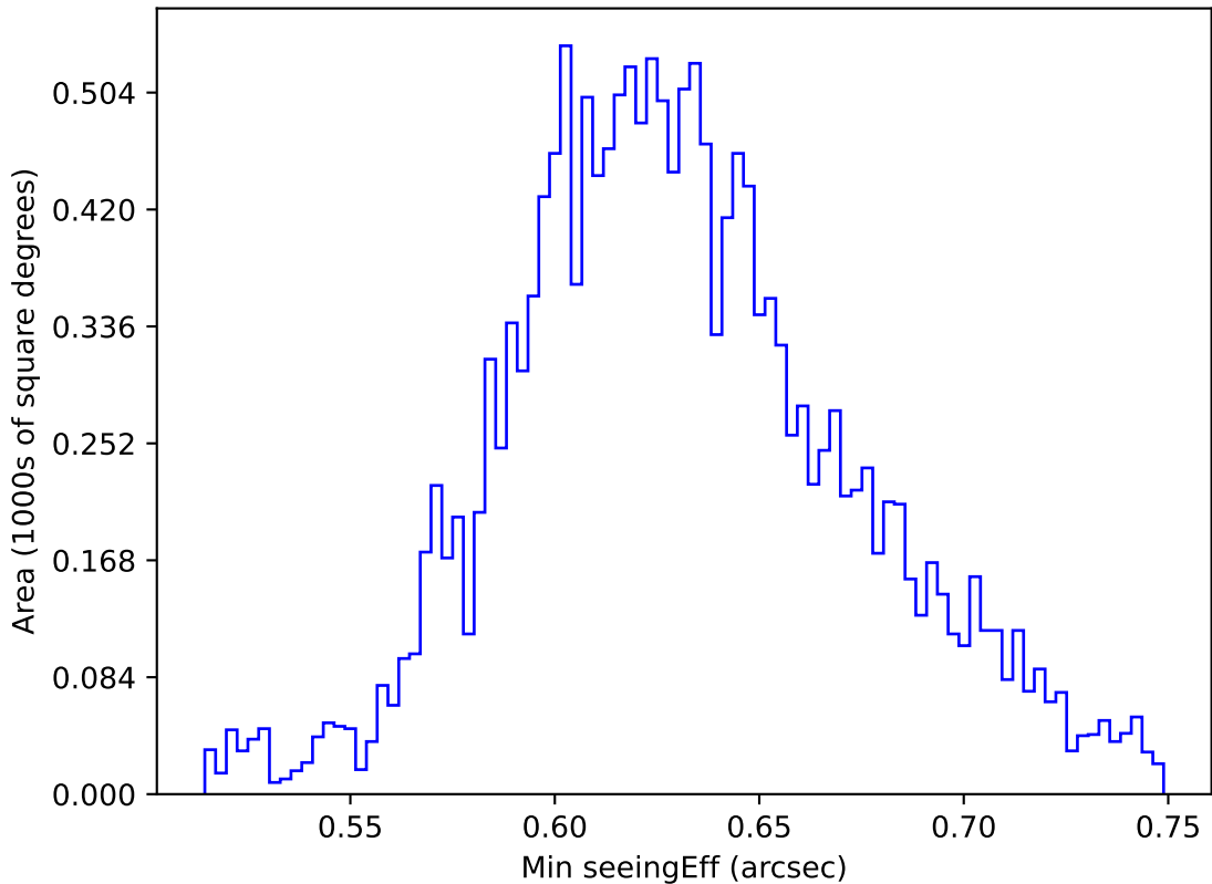
internal_u_expt60_nscale0.9v3.4_10yrs WFD y band: Min seeingEff
