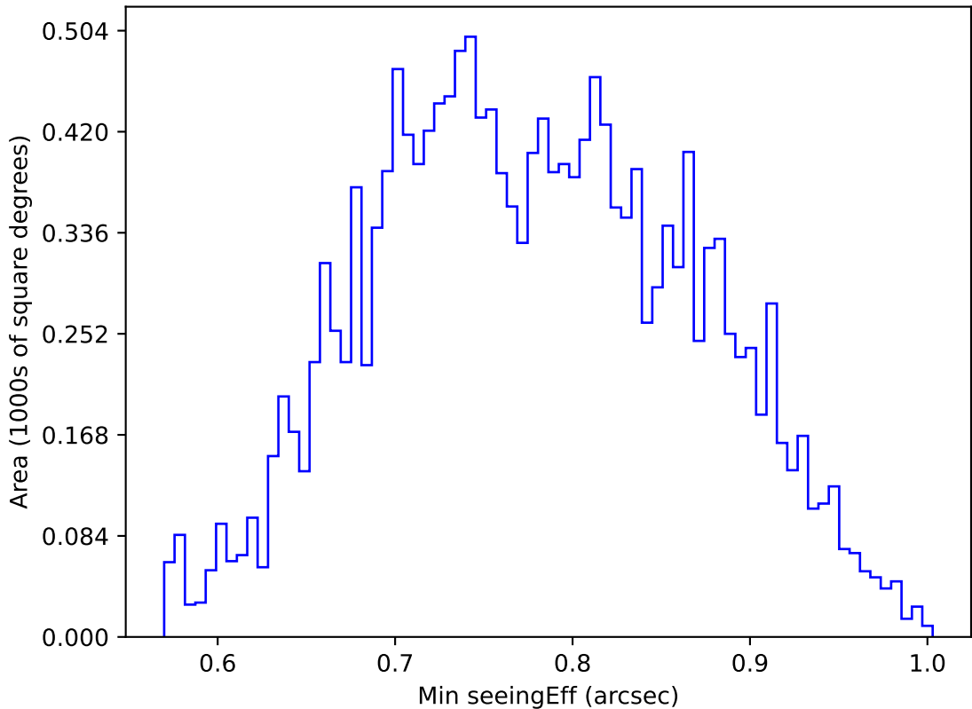
internal_u_expt60_nscale0.9v3.4_10yrs WFD u band: Min seeingEff
