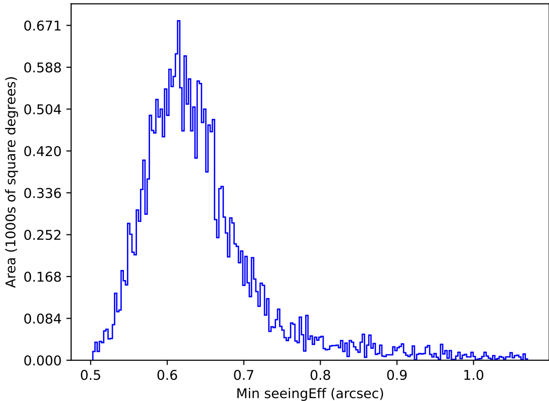
internal_u_expt60_nscale0.9v3.4_10yrs All sky r band: Min seeingEff
