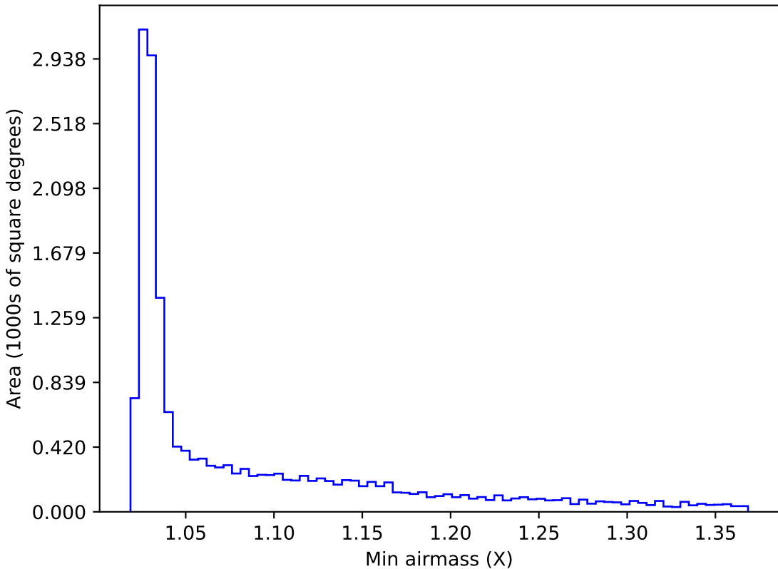
internal_u_expt60_nscale0.9v3.4_10yrs WFD z band: Min airmass
