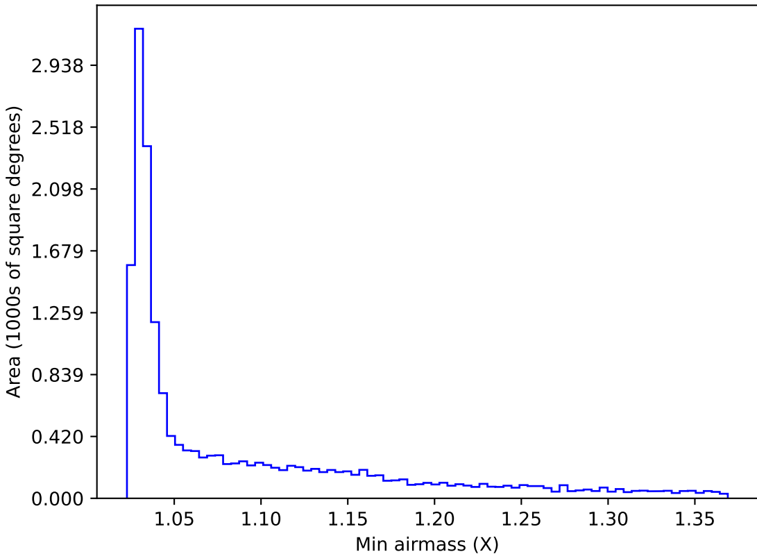
internal_u_expt60_nscale0.9v3.4_10yrs WFD y band: Min airmass
