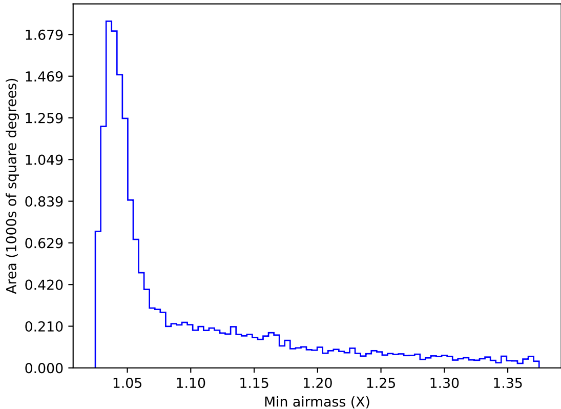
internal_u_expt60_nscale0.9v3.4_10yrs WFD u band: Min airmass
