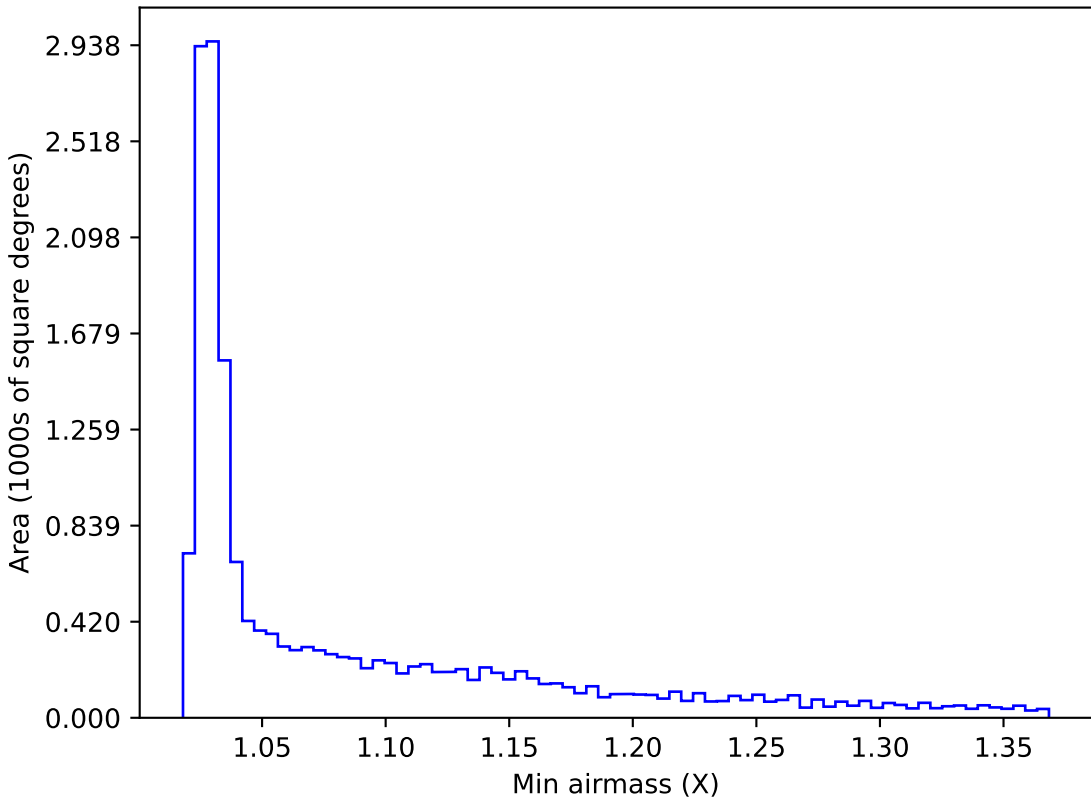
internal_u_expt60_nscale0.9v3.4_10yrs WFD i band: Min airmass
