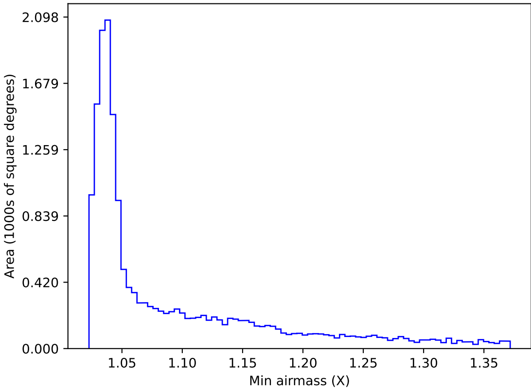
internal_u_expt60_nscale0.9v3.4_10yrs WFD g band: Min airmass
