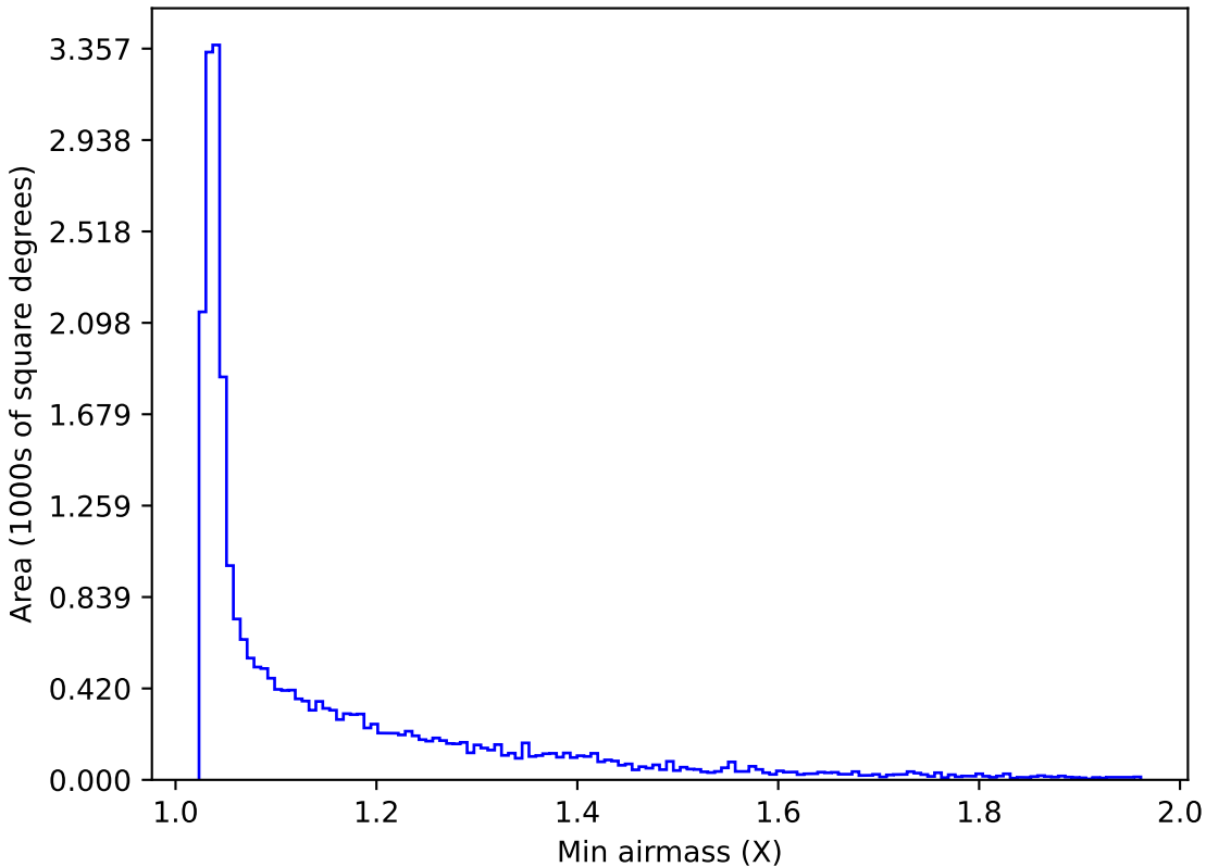
internal_u_expt60_nscale0.9v3.4_10yrs All sky g band: Min airmass
