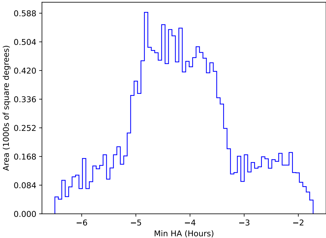
internal_u_expt60_nscale0.9v3.4_10yrs WFD g band: Min HA
