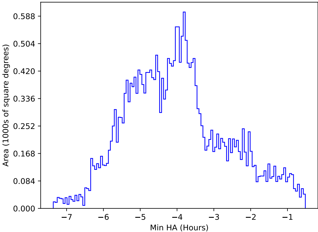
internal_u_expt60_nscale0.9v3.4_10yrs All sky z band: Min HA
