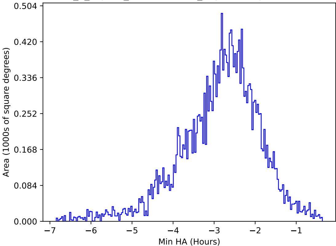
internal_u_expt60_nscale0.9v3.4_10yrs All sky u band: Min HA
