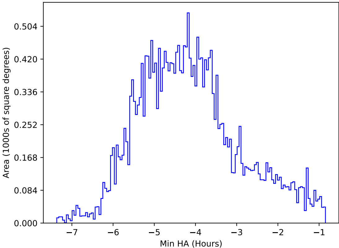
internal_u_expt60_nscale0.9v3.4_10yrs All sky r band: Min HA
