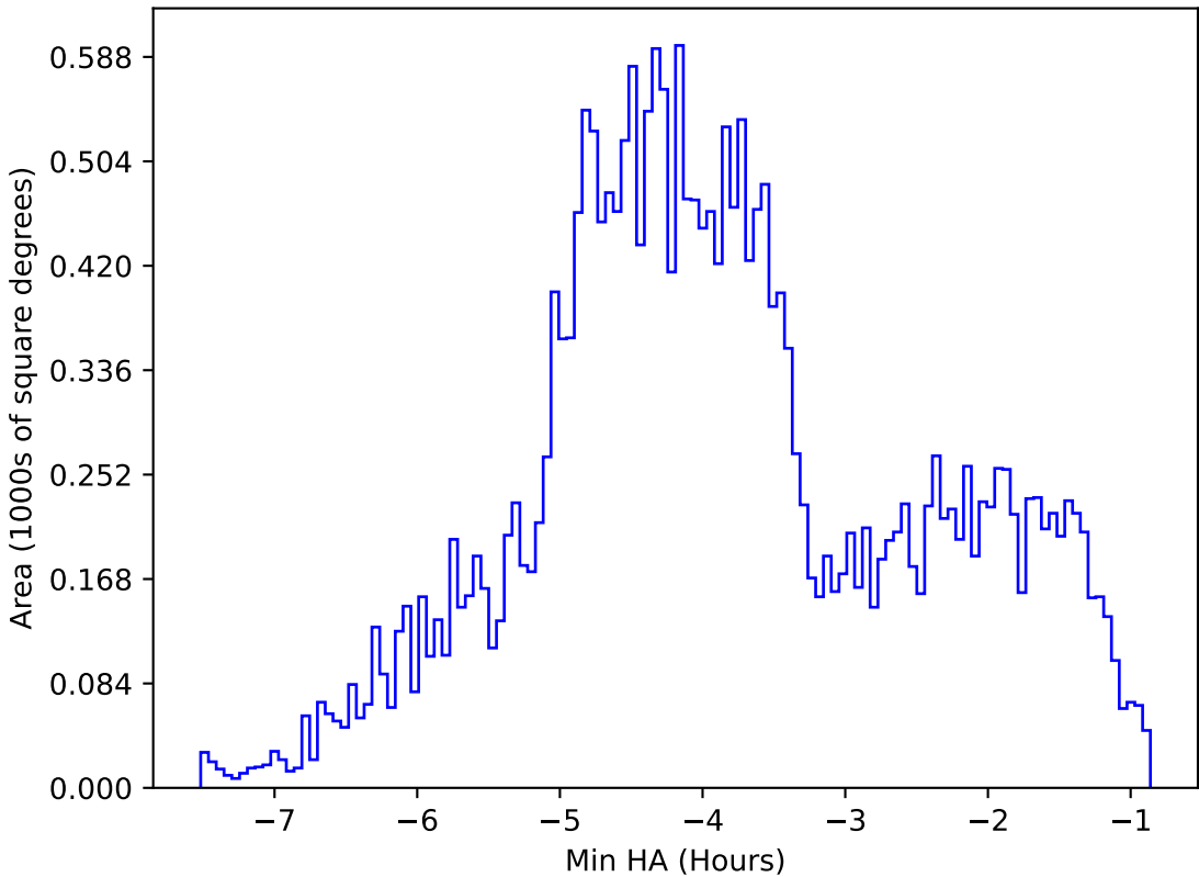
internal_u_expt60_nscale0.9v3.4_10yrs All sky g band: Min HA
