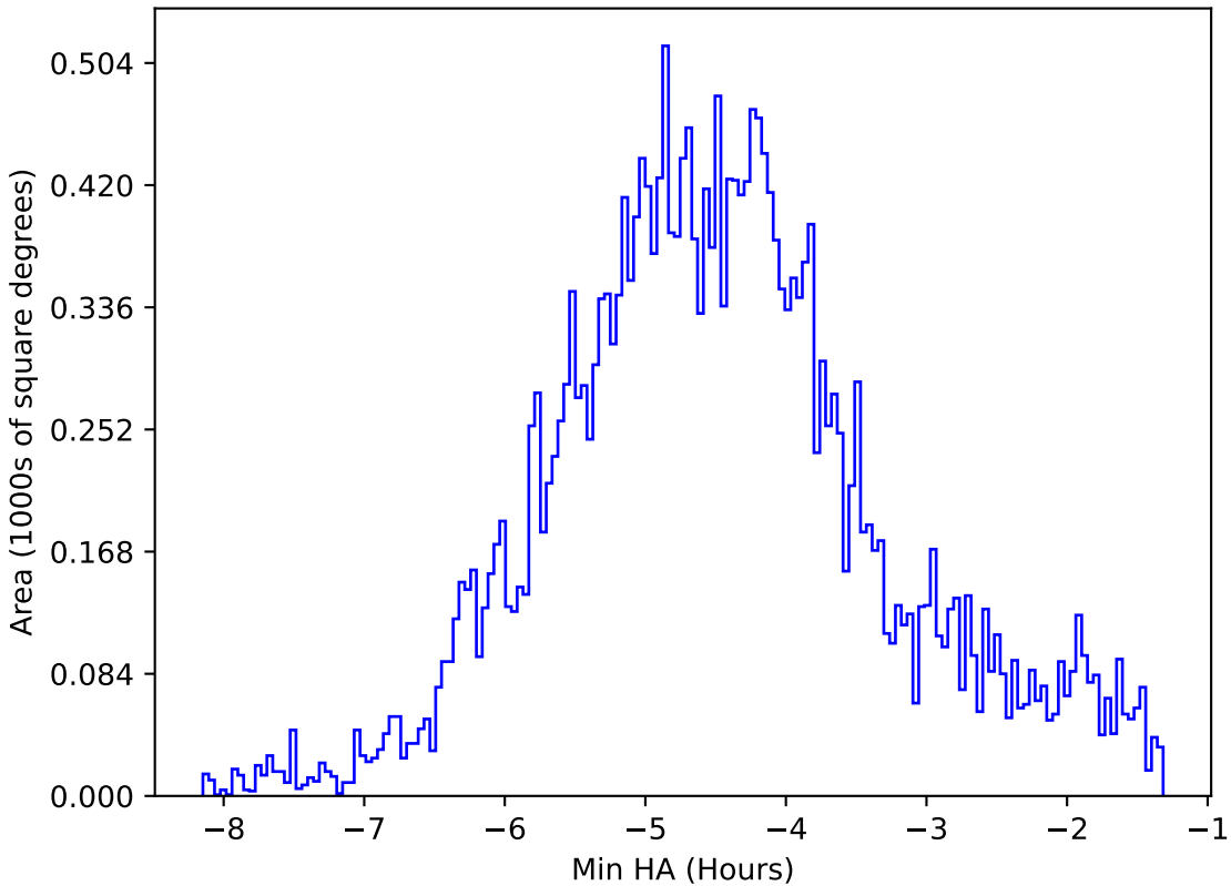
internal_u_expt60_nscale0.9v3.4_10yrs All sky all bands: Min HA
