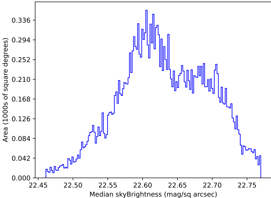
internal_u_expt60_nscale0.9v3.4_10yrs Yr 1 u band: Median skyBrightness
